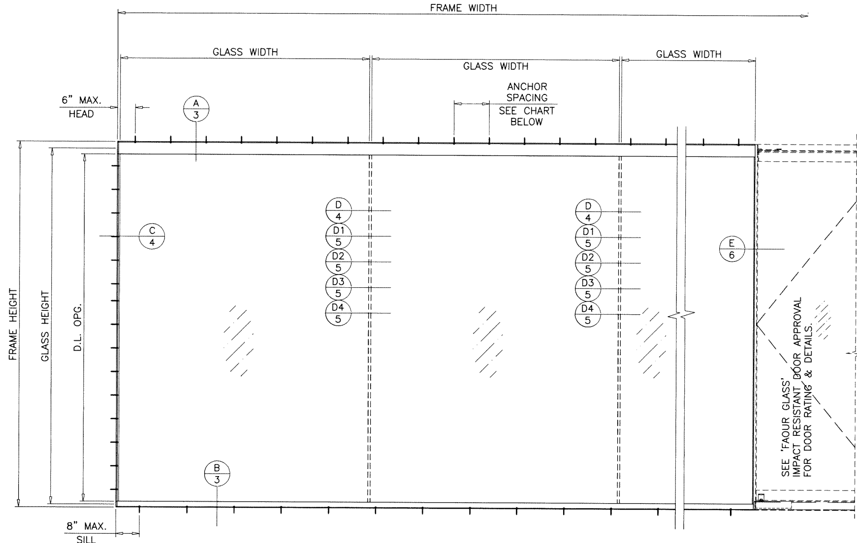
TYPICAL ELEVATIONS
